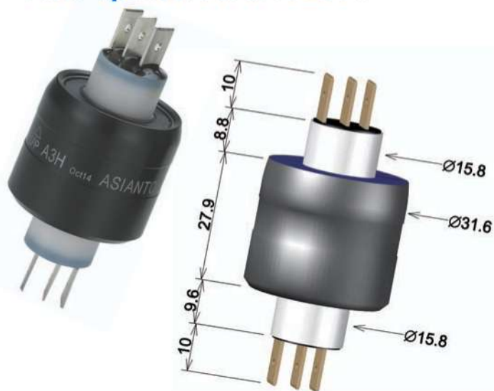
A3H 3poles/30A/AC250V
