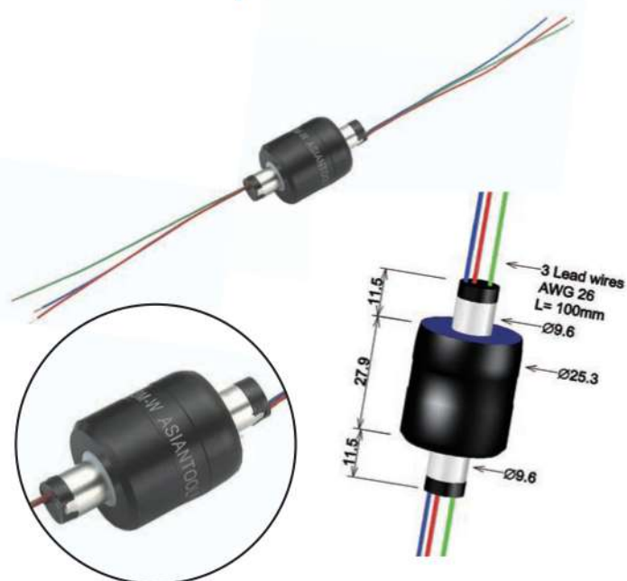
A3M-W 3poles/4A/AC250V
